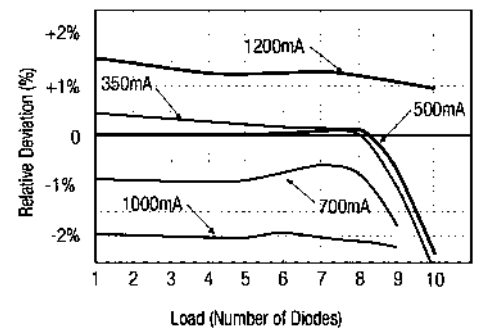
Output Current Accuracy/Load
