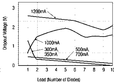
Dropout Voltage/Load
