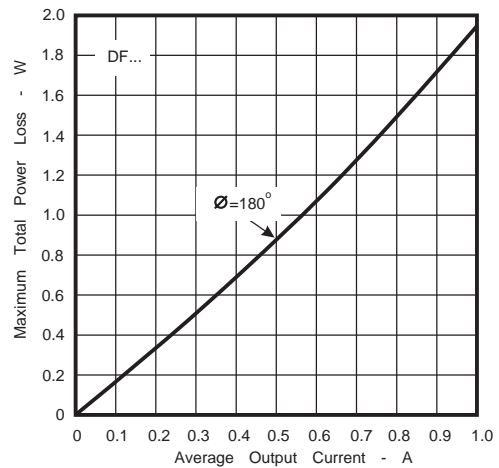
Fig. 2 - Power Loss Characteristics
