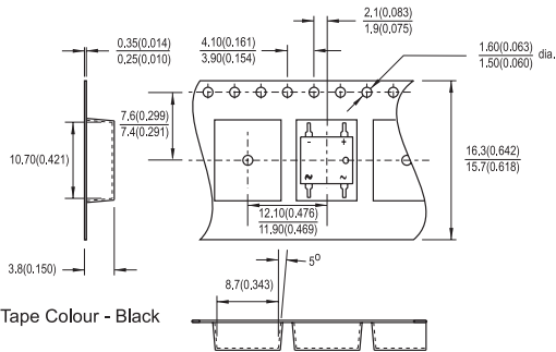
Tape Reel Dimensions for DF..TRR16
