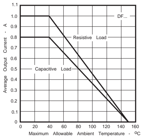
Fig. 3 - Current Ratings
