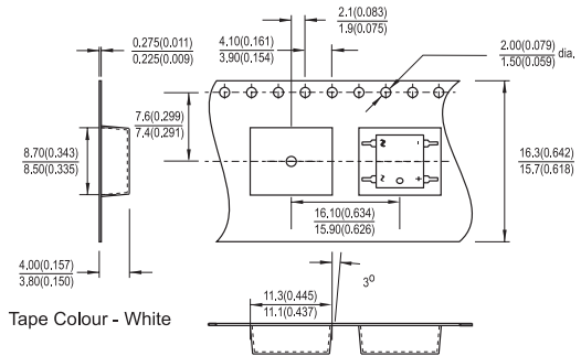
Tape Reel Dimensions for DF..TR16
