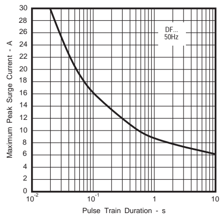
Fig. 4 - Non-Repetitive Surge Ratings
