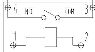
(Bottom View) 底视
