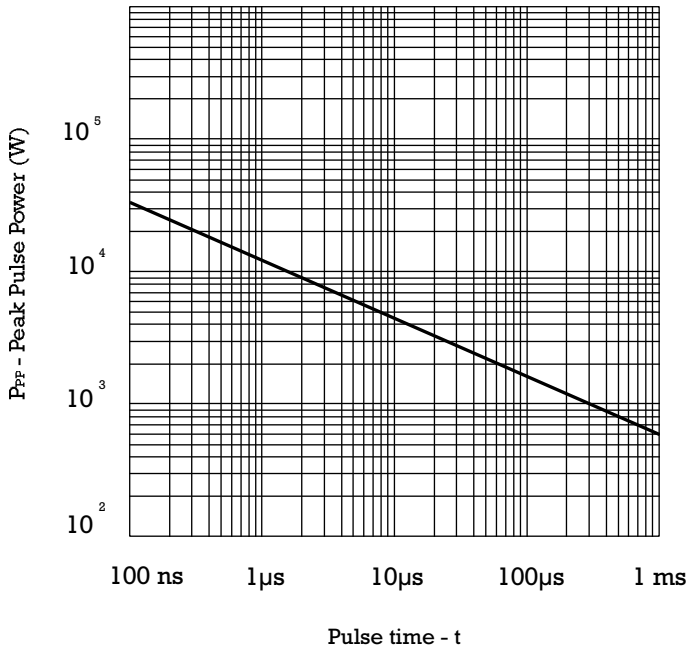
PEAK PULSE POWER RATING CURVE
