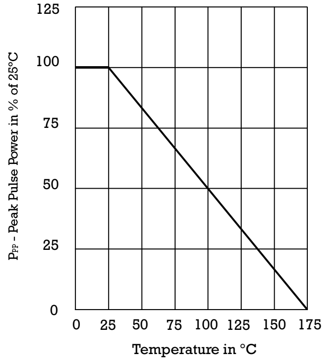
DERATING CURVE
