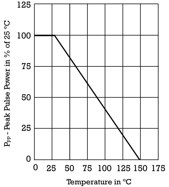
DERATING CURVE
