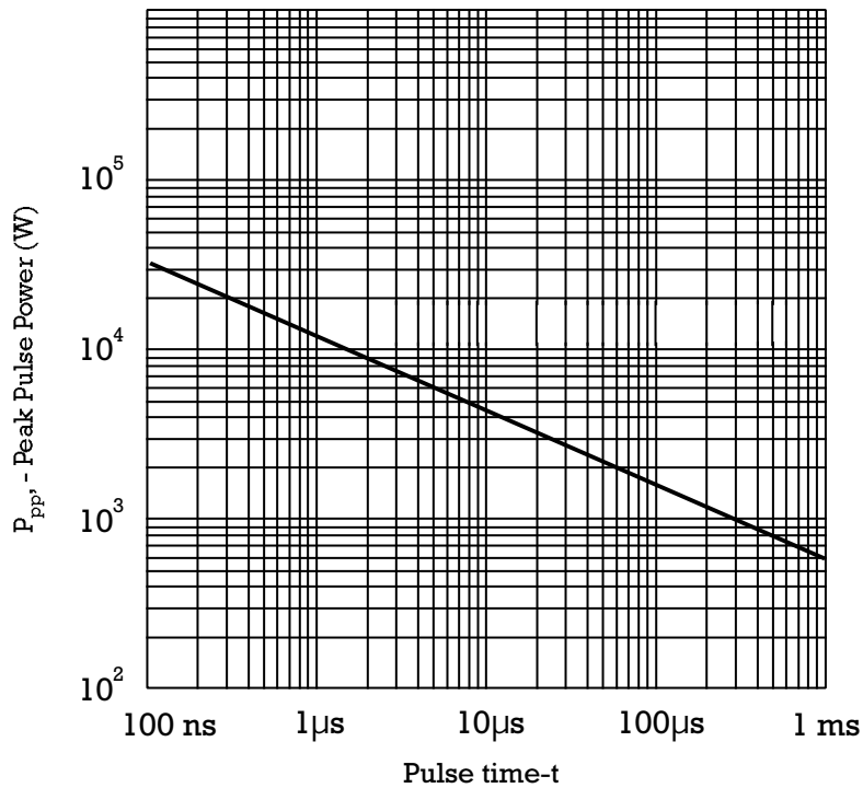
PEAK PULSE POWER RATING CURVE
