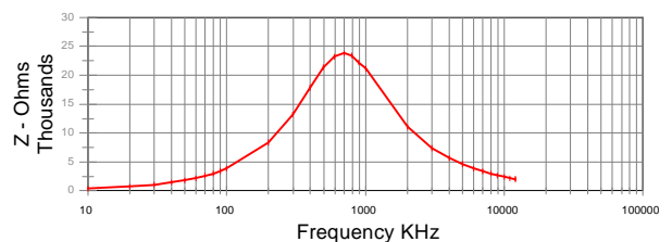
Impedance Curve
