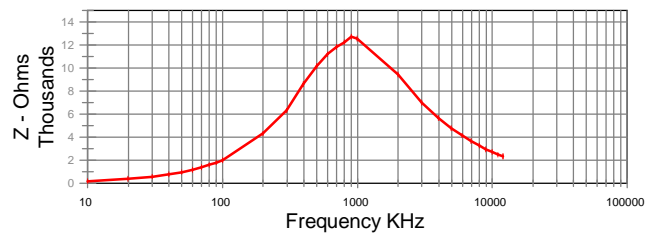
Impedance Curve
