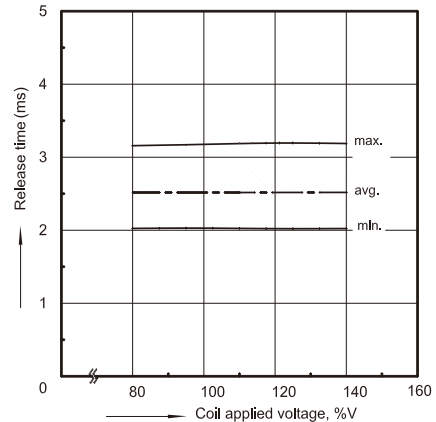
Release time
